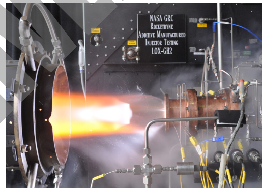
Top: NASA Glenn engineers installing Aerojet Rocketdyne hardware on the test stand. Bottom: Rocket injector assembly built by AM being hot-fire tested at NASA Glenn.
